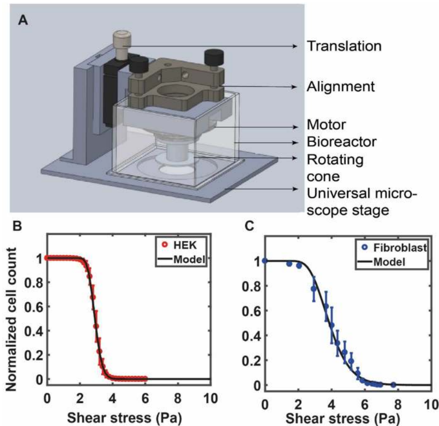
FIGURE 4 | (A) The custom fluid shear device used by Maan et al. (2018) is shown in (A). The device is mounted on a microscope for real-time visualization of cells under shear. The device consists of a 1^\circ cone attached to a motor that is used to apply increasing shear stress on cells cultured on a petri dish (see Maan et al., 2018 for details). RPM of the motor is controlled by a computer via a feedback loop. A bioreactor, placed around the device, is used to maintain physiological conditions. The number of adherent cells is counted at each value of shear and is used to quantify the deadhesion strength. (B) The curve shows experimental data for HEK cells against the model prediction of Equation (7) with the values of \sigma_o and s obtained from a best-fit analysis: \sigma_o = 2.91 , \sqrt{2}s = 0.16 (HEK). (C) Experimental data for 3T3 fibroblast cells against the model prediction of Equation (7) with the values of \sigma_o and s obtained from a best-fit analysis: \sigma_o = 3.85 , \sqrt{2}s = 0.35 . (B,C) Are reprinted with permission from IOP Science, Physical Biology (Maan et al., 2018).
